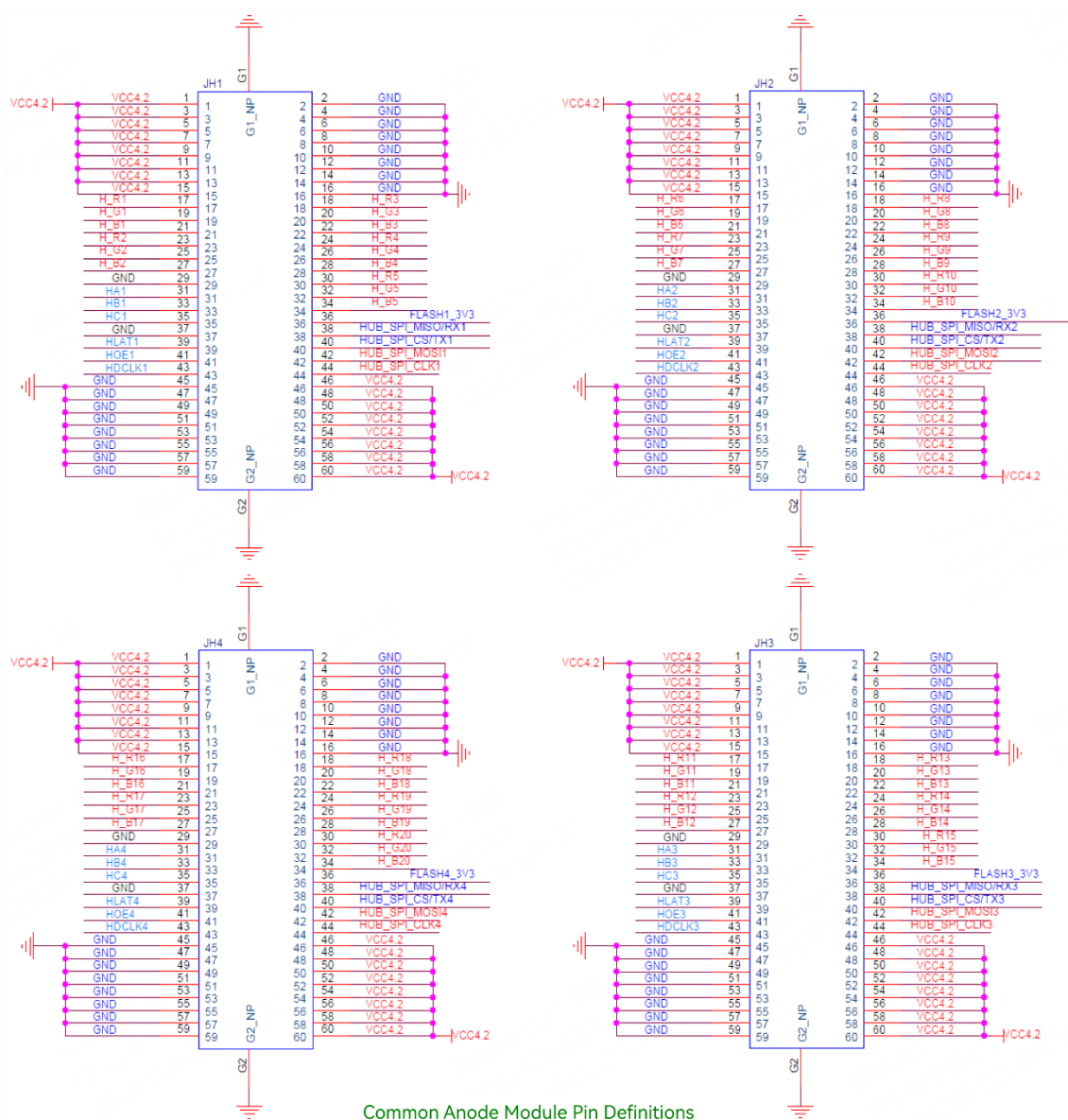
Pin Definitions (Taking JH1 as an example)
