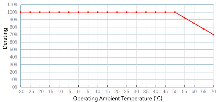
Temperature Derating Curve
