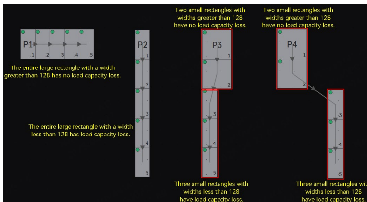
Figure 11-1 Load capacity loss example
