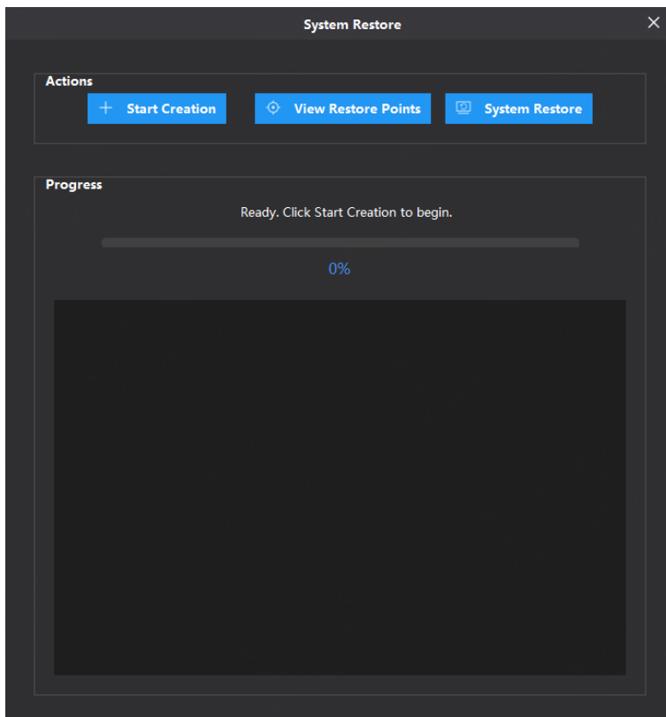
Figure 7-6 System restore
