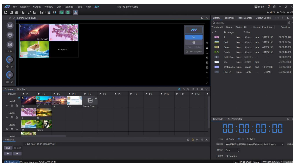
Figure 3-1 User interface
