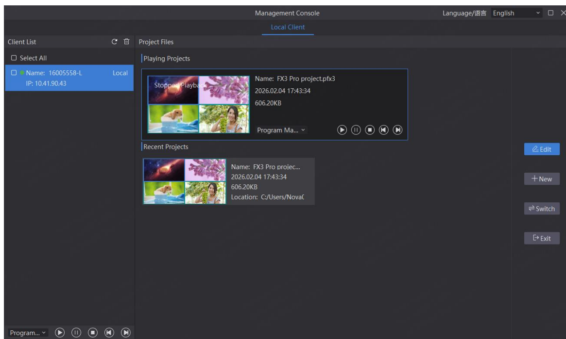
Figure 10-1 Management console
