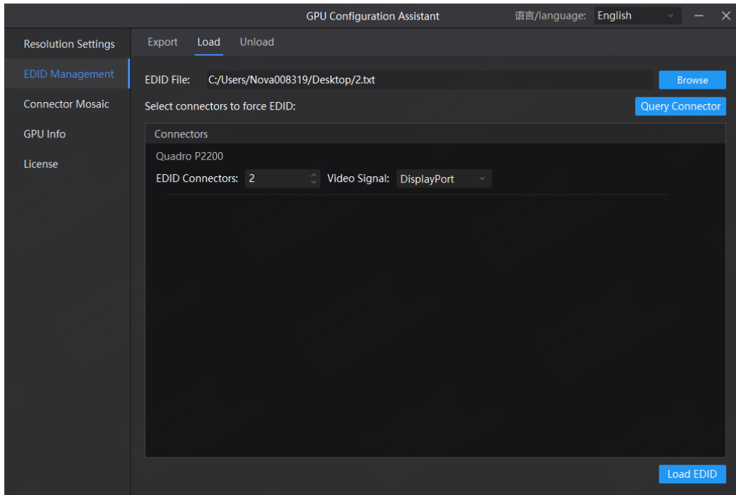
Figure 7-9 Load EDID
