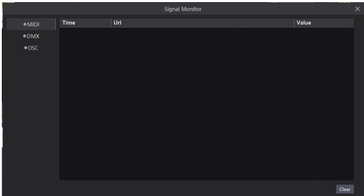
Figure 6-11 Signal monitoring
