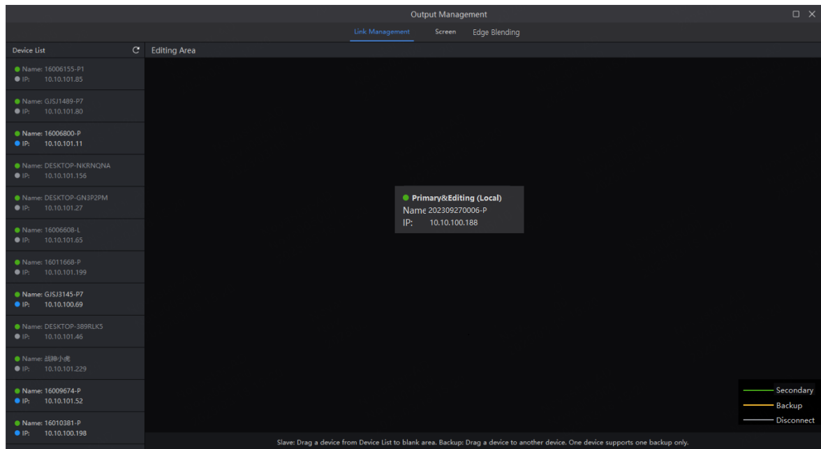
Figure 5-2 Link settings
