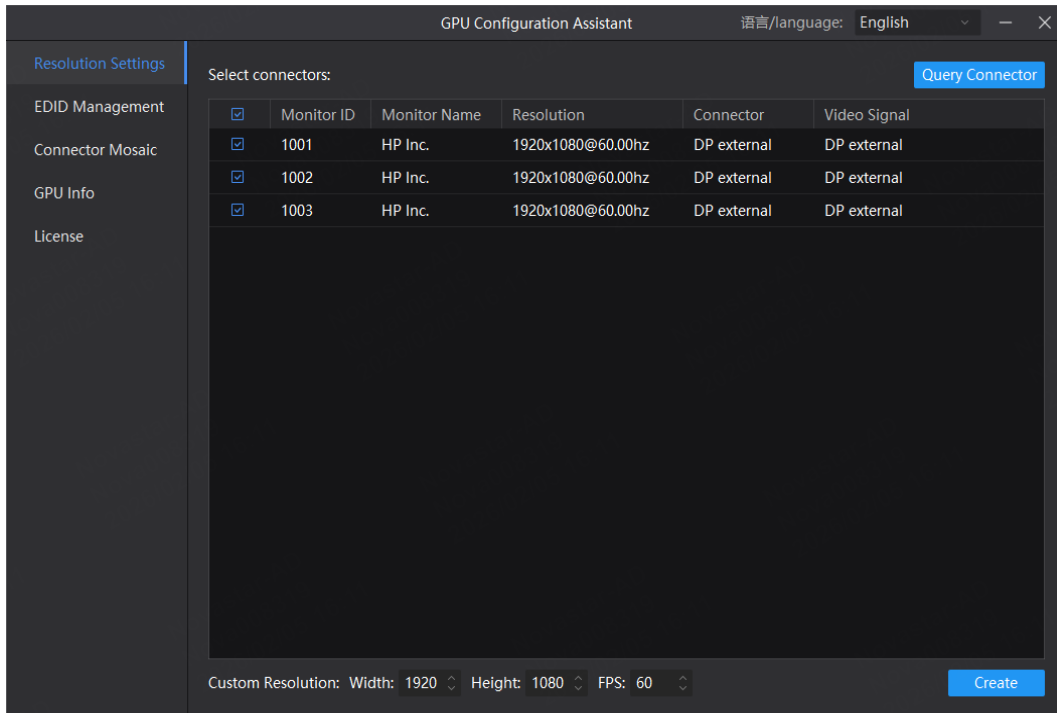
Figure 7-7 Configure resolution
