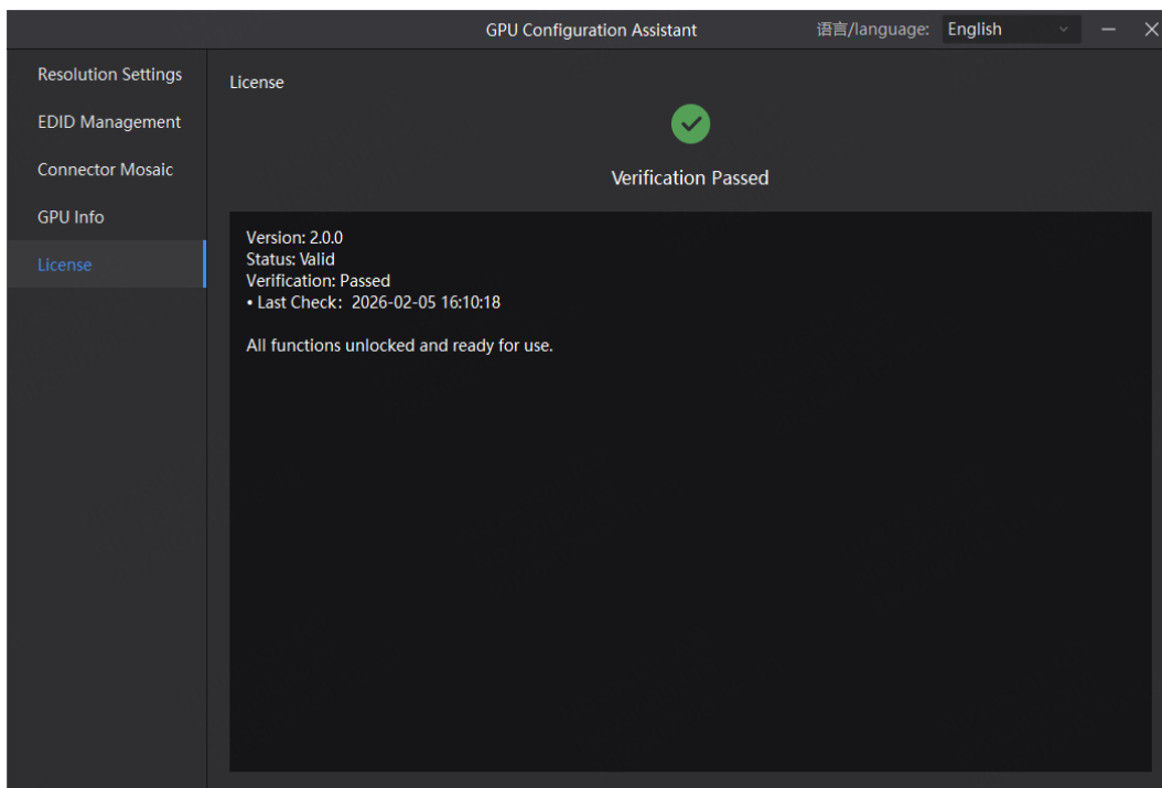
Figure 7-14 License management
