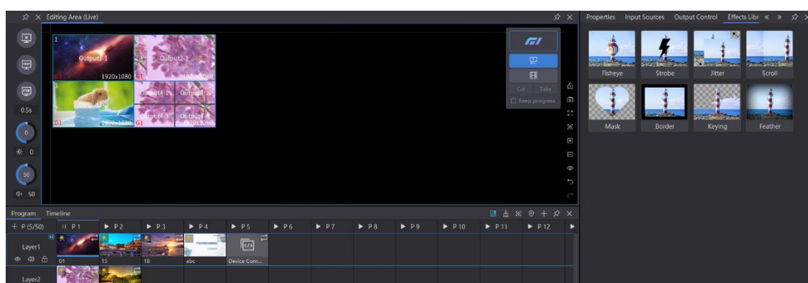
Figure 4-57 Add effects
