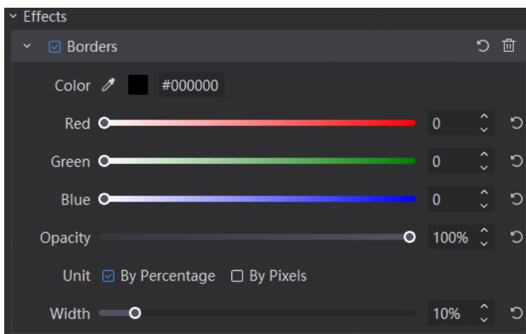
Figure 4-62 Border effect
