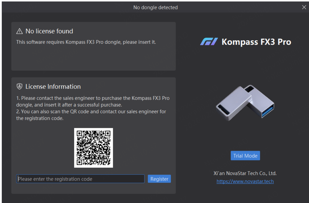
Figure 1-4 Dongle detection
