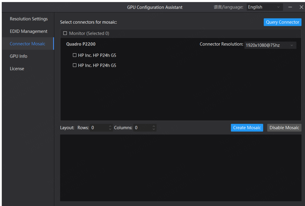
Figure 7-12 Create mosaic
