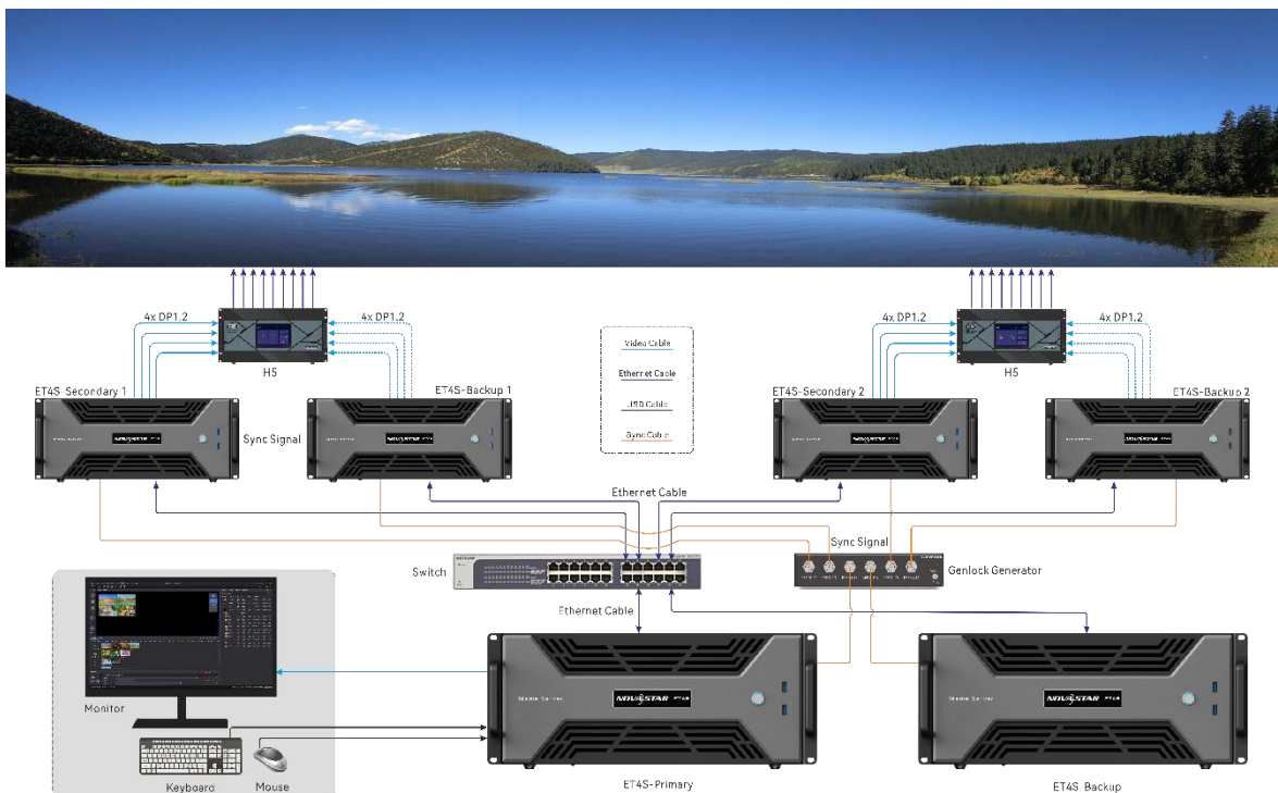
Figure 5-1 Application scenarios
