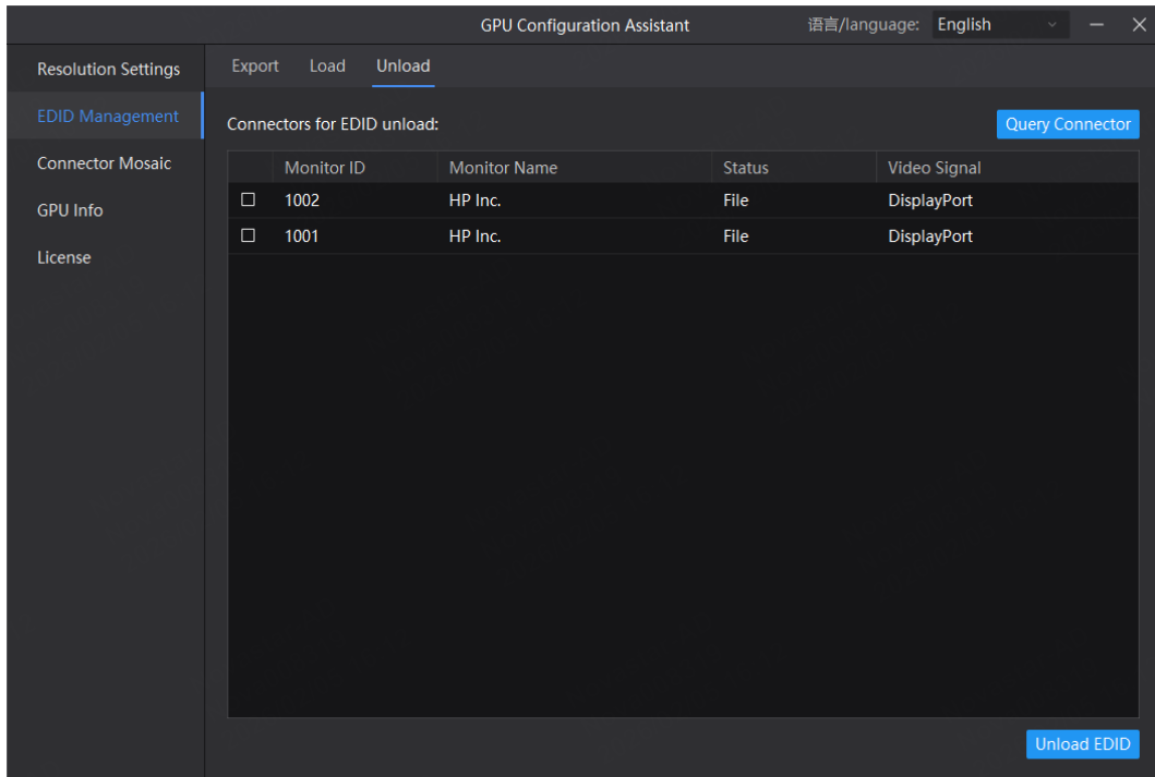
Figure 7-10 Unload EDID
