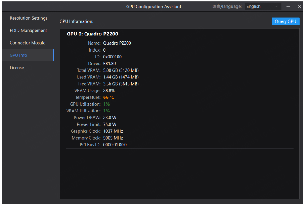
Figure 7-13 GPU info
