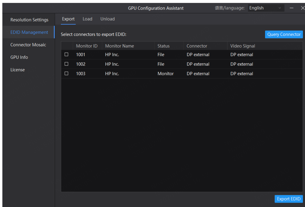
Figure 7-8 Export EDID
