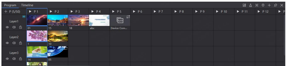
Figure 3-8 Program management
