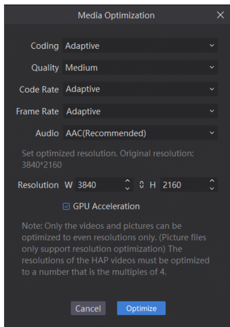
Figure 4-5 Media optimization
