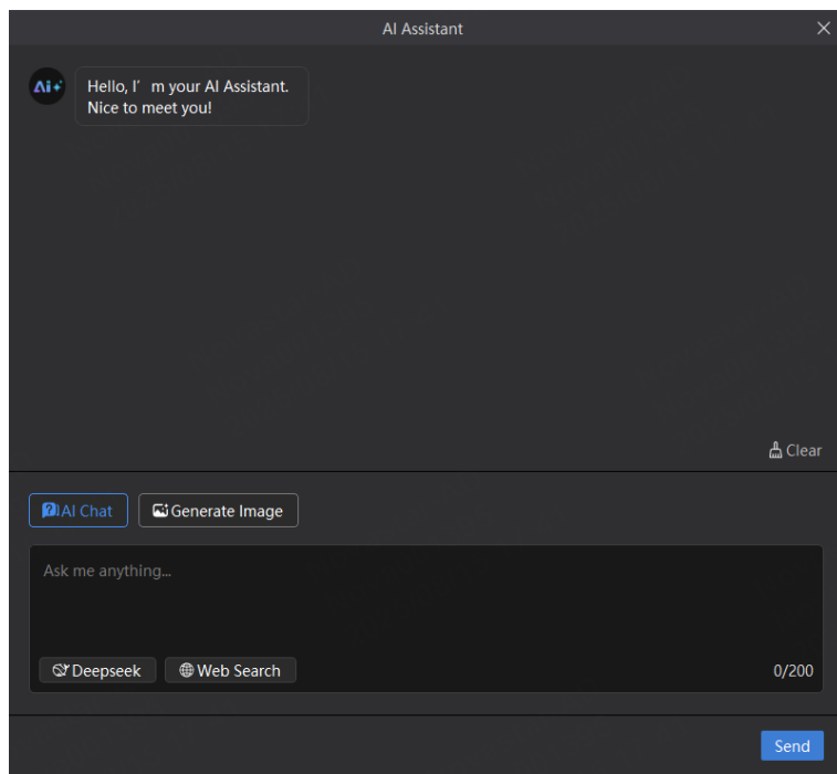
Figure 9-5 AI assistant
