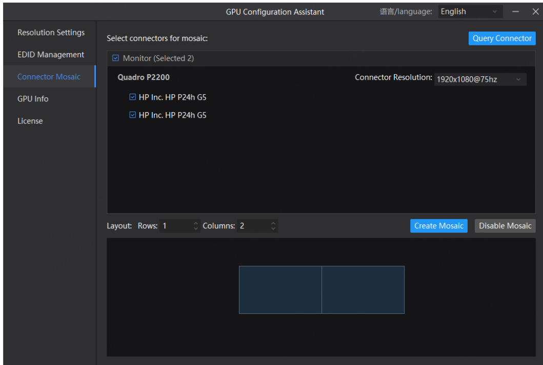
Figure 7-11 Query connectors
