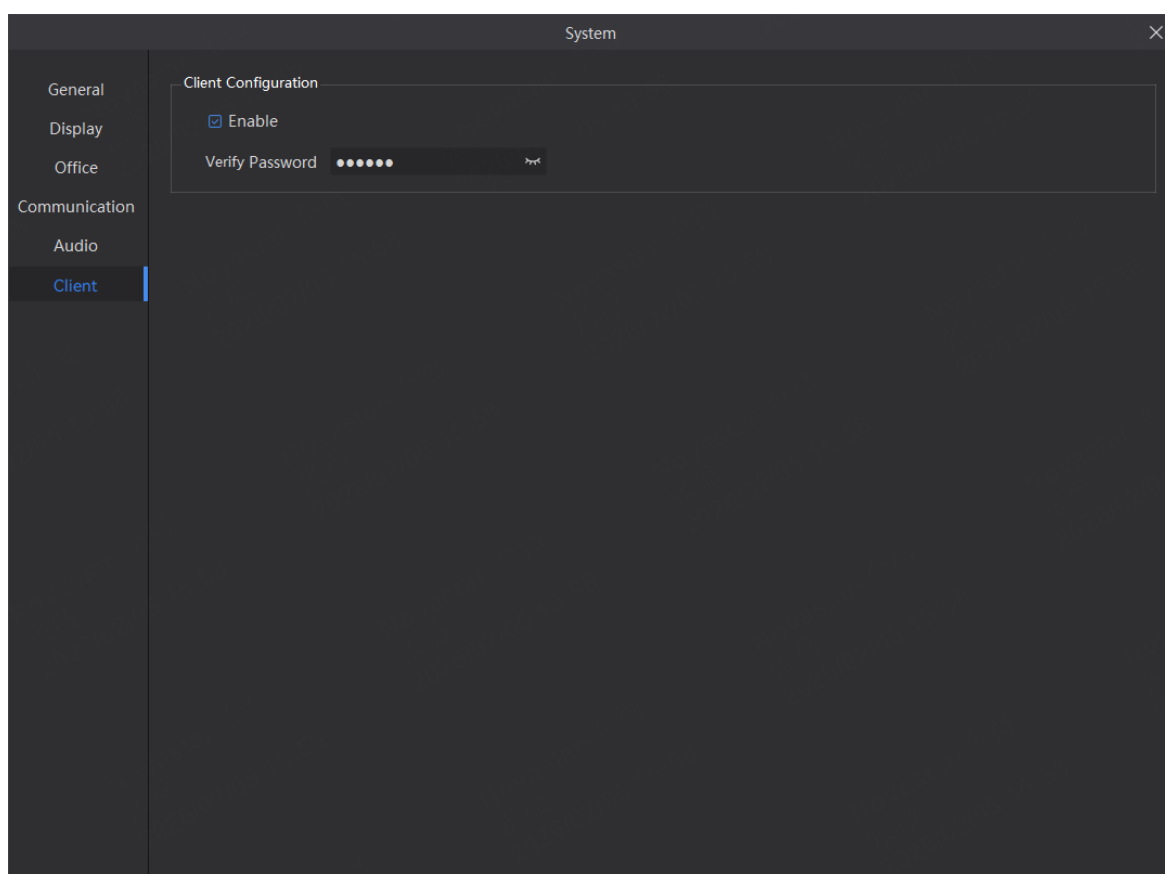
Figure 6-7 Client
