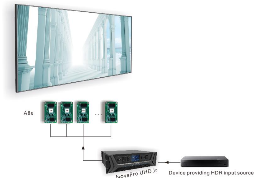
Figure 5-21 System architecture
