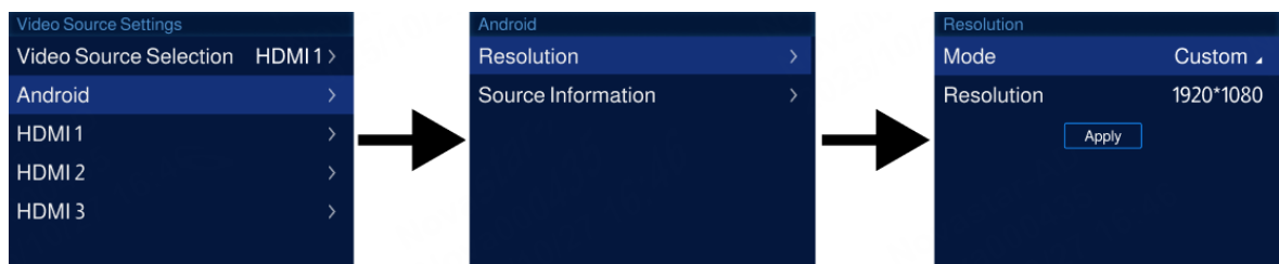
Figure 2-8 Resolution (Android)
