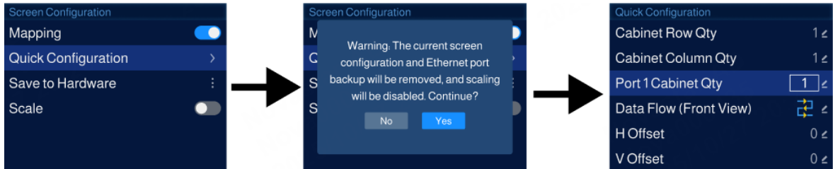
Figure 2-13 Quick configuration
