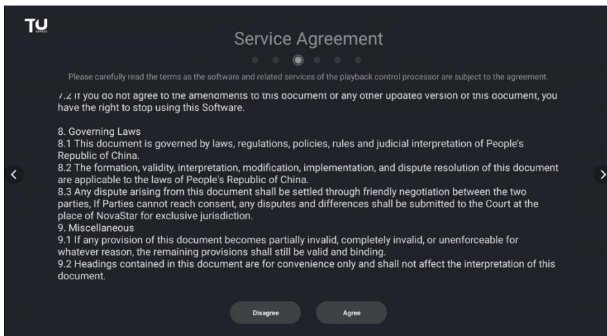
Figure 3-5 Service agreement
