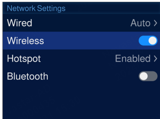
Figure 2-21 Wireless network
