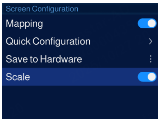
Figure 2-15 Enable scaling
