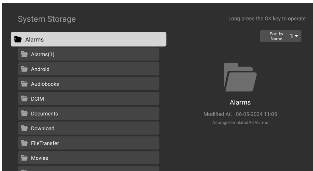
Figure 3-39 Pasting completed
