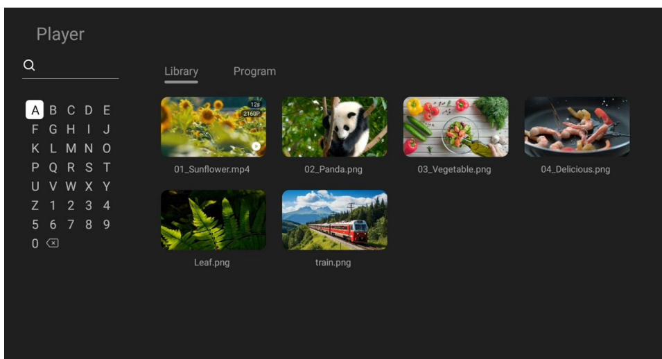
Figure 3-55 Search
