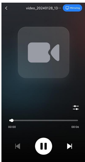
Figure 3-14 Display video
