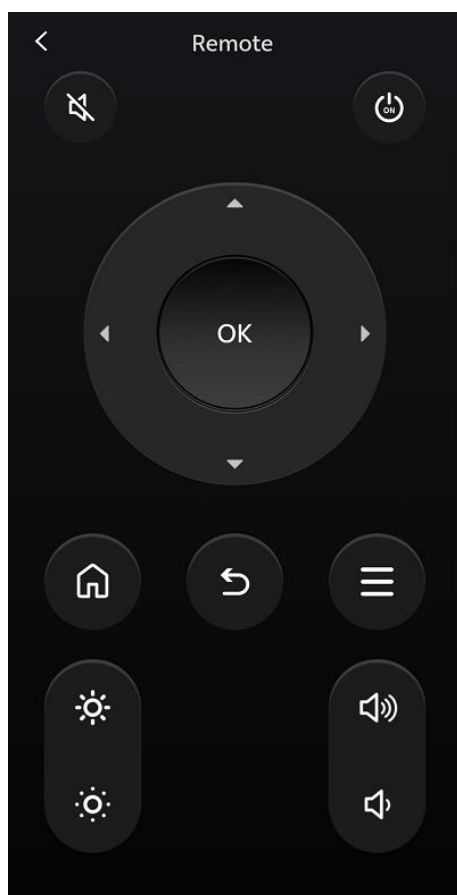
Figure 3-17 Remote
