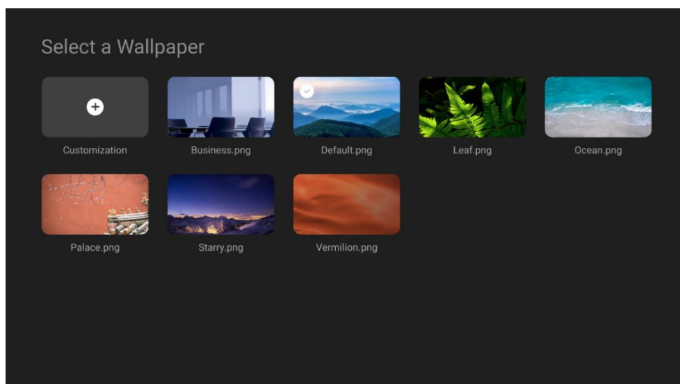
Figure 3-73 Wallpaper
