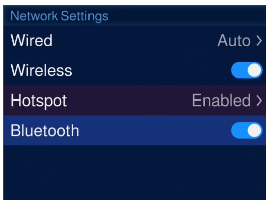
Figure 2-23 Bluetooth
