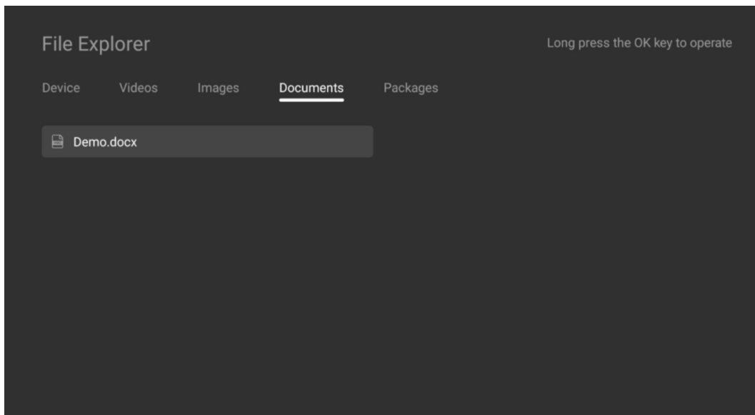
Figure 3-43 Documents
