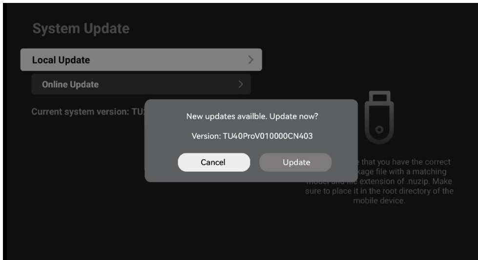
Figure 3-78 Local Update
