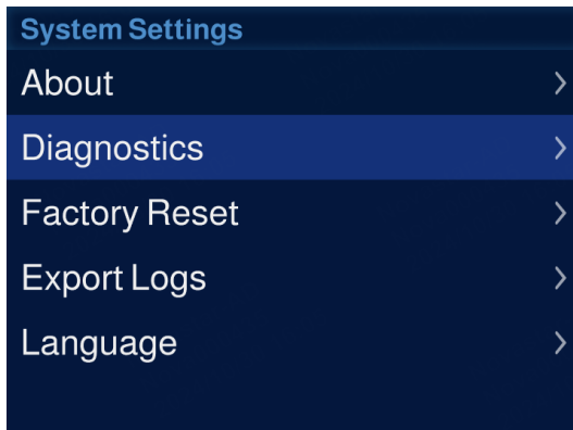
Figure 2-30 Diagnostics
