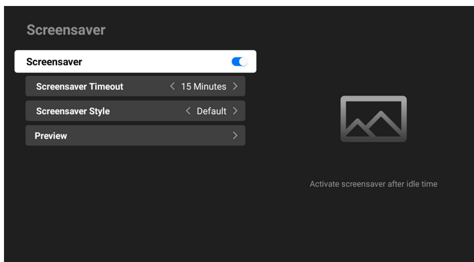
Figure 3-71 Screensaver
