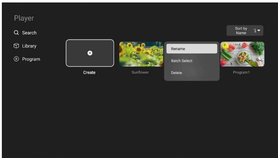
Figure 3-49 Media library
