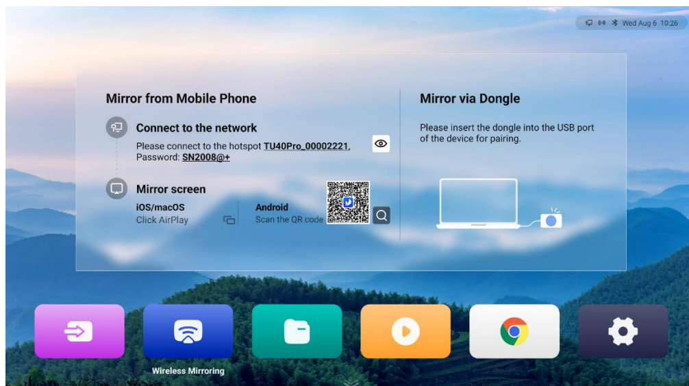
Figure 3-11 Wireless mirroring
