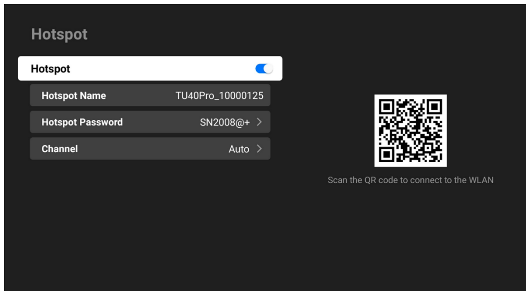
Figure 3-60 Hotspot
