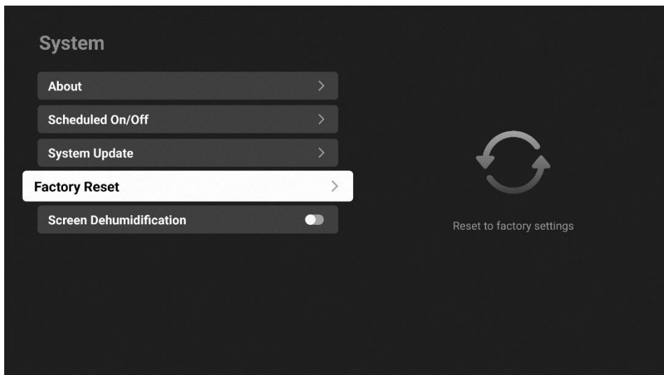
Figure 3-80 Factory reset
