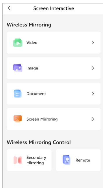
Figure 3-12 Screen interactive
