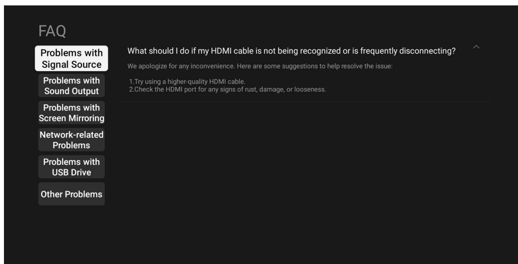
Figure 3-35 FAQ
