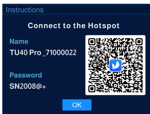
Figure 2-2 Hotspot connection
