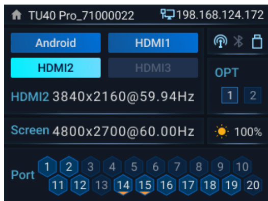
Figure 2-3 Home screen
