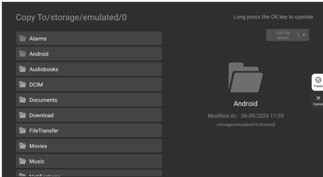
Figure 3-38 Paste
