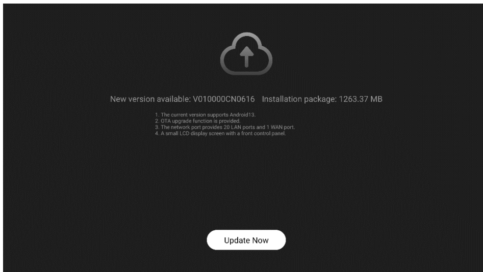
Figure 3-79 Online update
