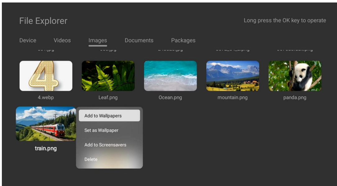
Figure 3-45 Images
