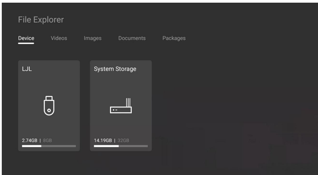
Figure 3-42 File explorer
