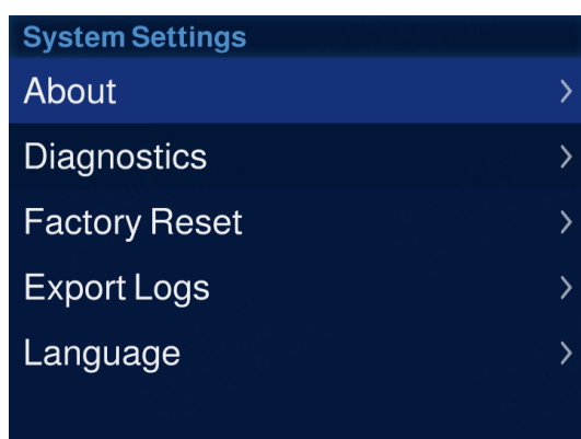
Figure 2-28 About
