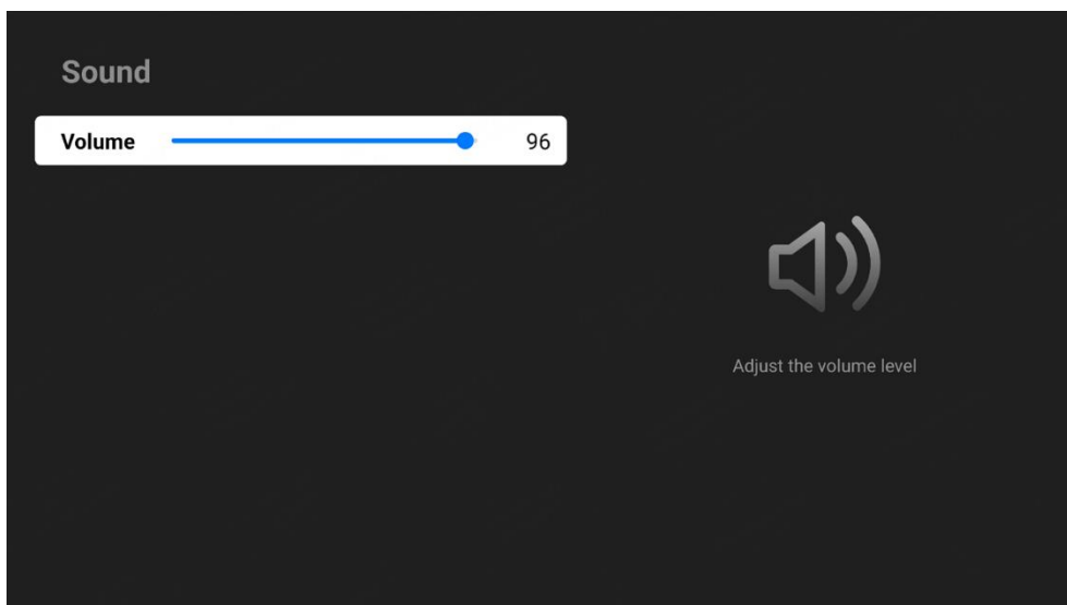
Figure 3-66 Sound settings
