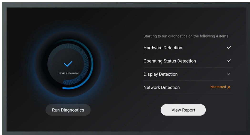
Figure 3-34 Diagnostic result
