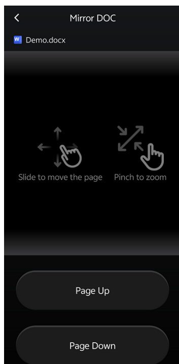
Figure 3-15 Display document
