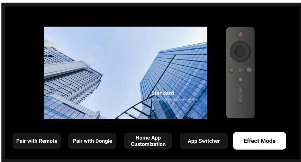
Figure 3-31 Effect mode
