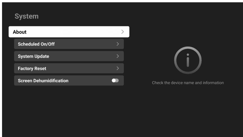
Figure 3-75 About
