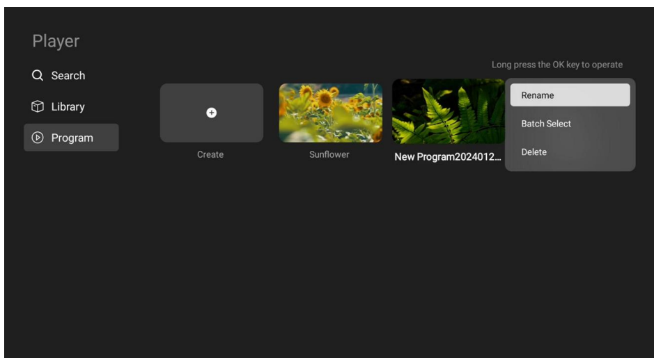
Figure 3-53 Program operations
