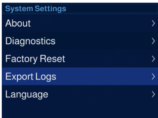
Figure 2-35 Export logs
