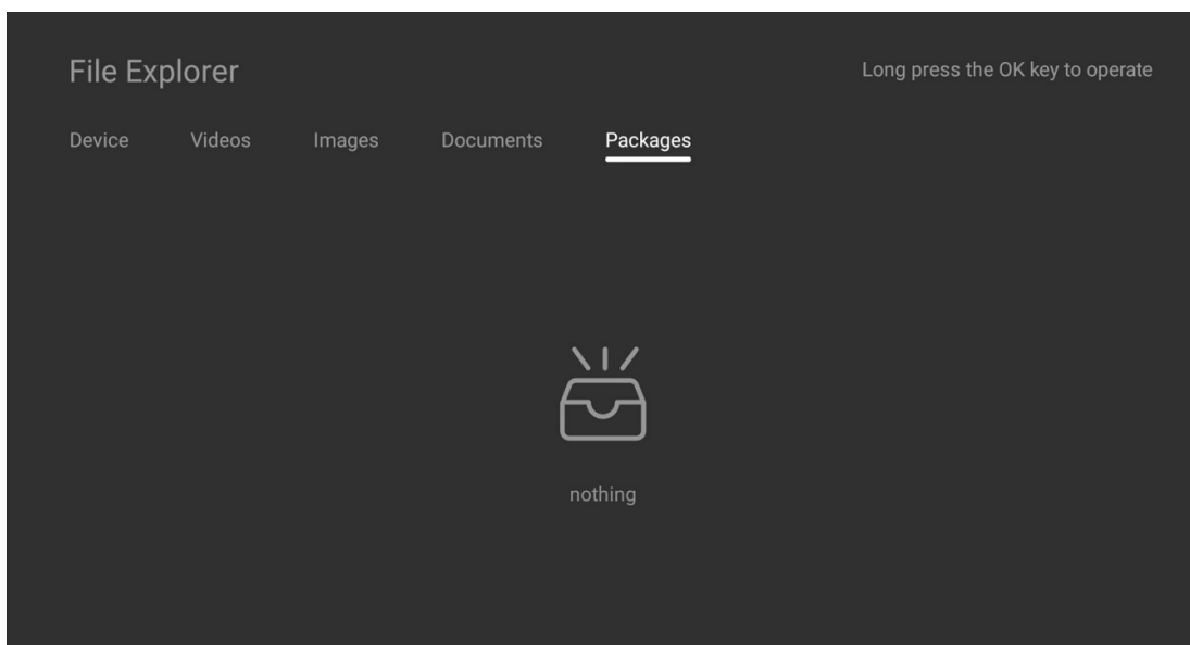
Figure 3-46 Packages
