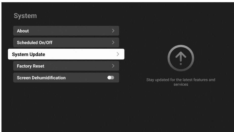
Figure 3-77 System update
