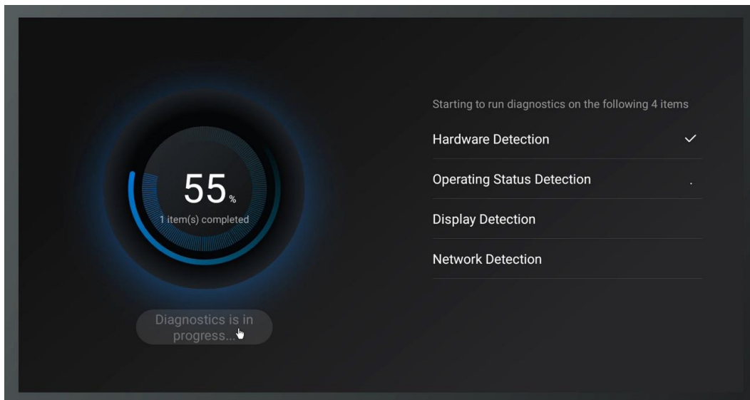
Figure 3-33 Running diagnostics
