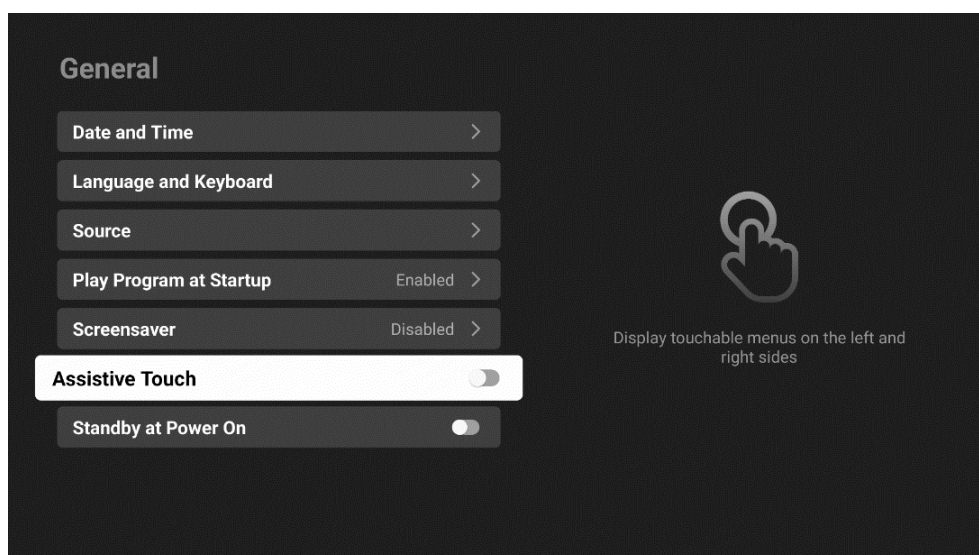
Figure 3-72 Assistive touch
