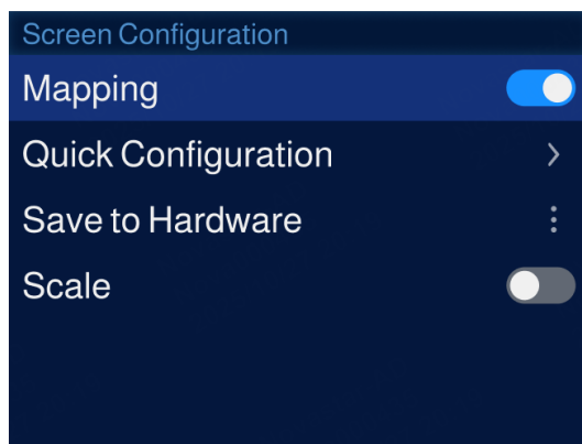
Figure 2-12 Enabling Mapping
