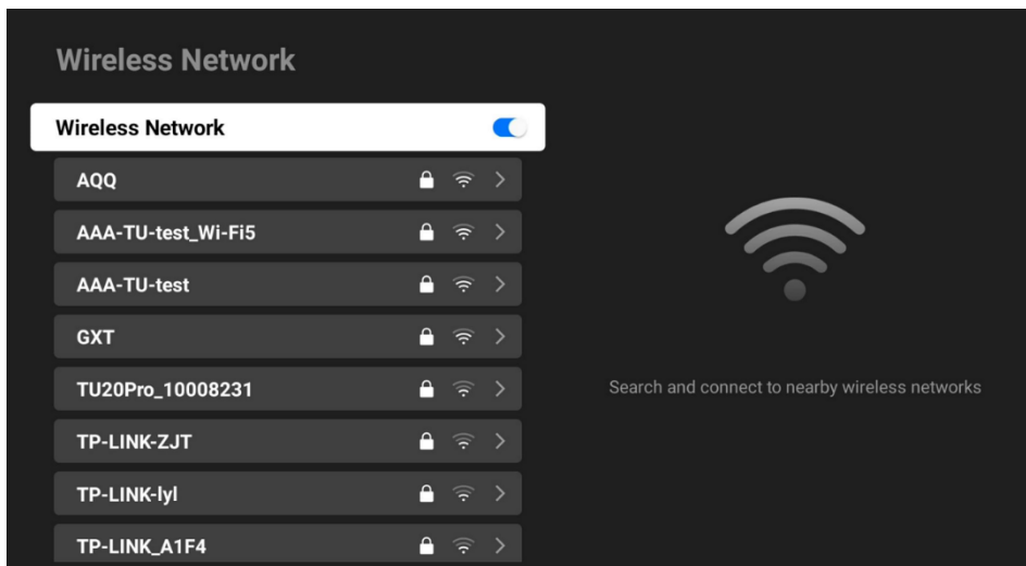
Figure 3-57 Wireless network
