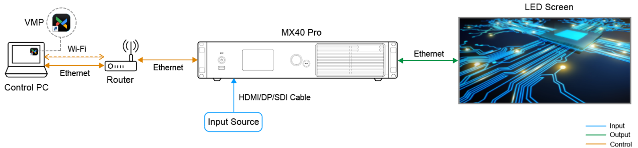
Figure 4-2 Connecting devices via LAN
