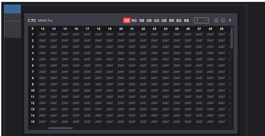
Figure 15-5 Pixel calibration coefficients
