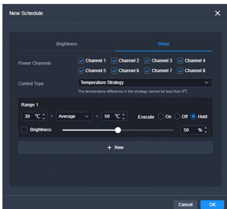
Figure 7-47 Create relay schedules
