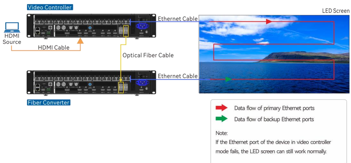
Figure 5-23 Backup between Ethernet and OPT ports
