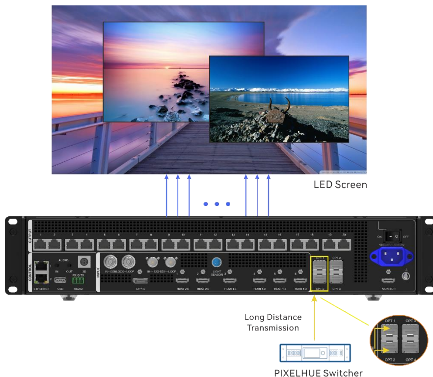
Figure 5-11 OPT input sources
